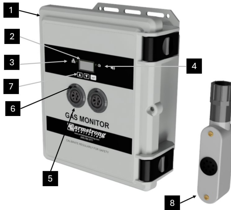
Figure 2-1: External View
