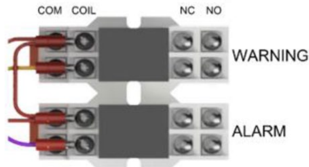
Figure 3-4: Relay Connections
