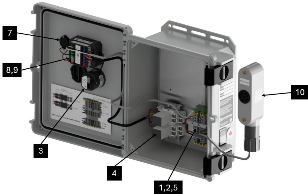
Figure 2-2: Internal View
