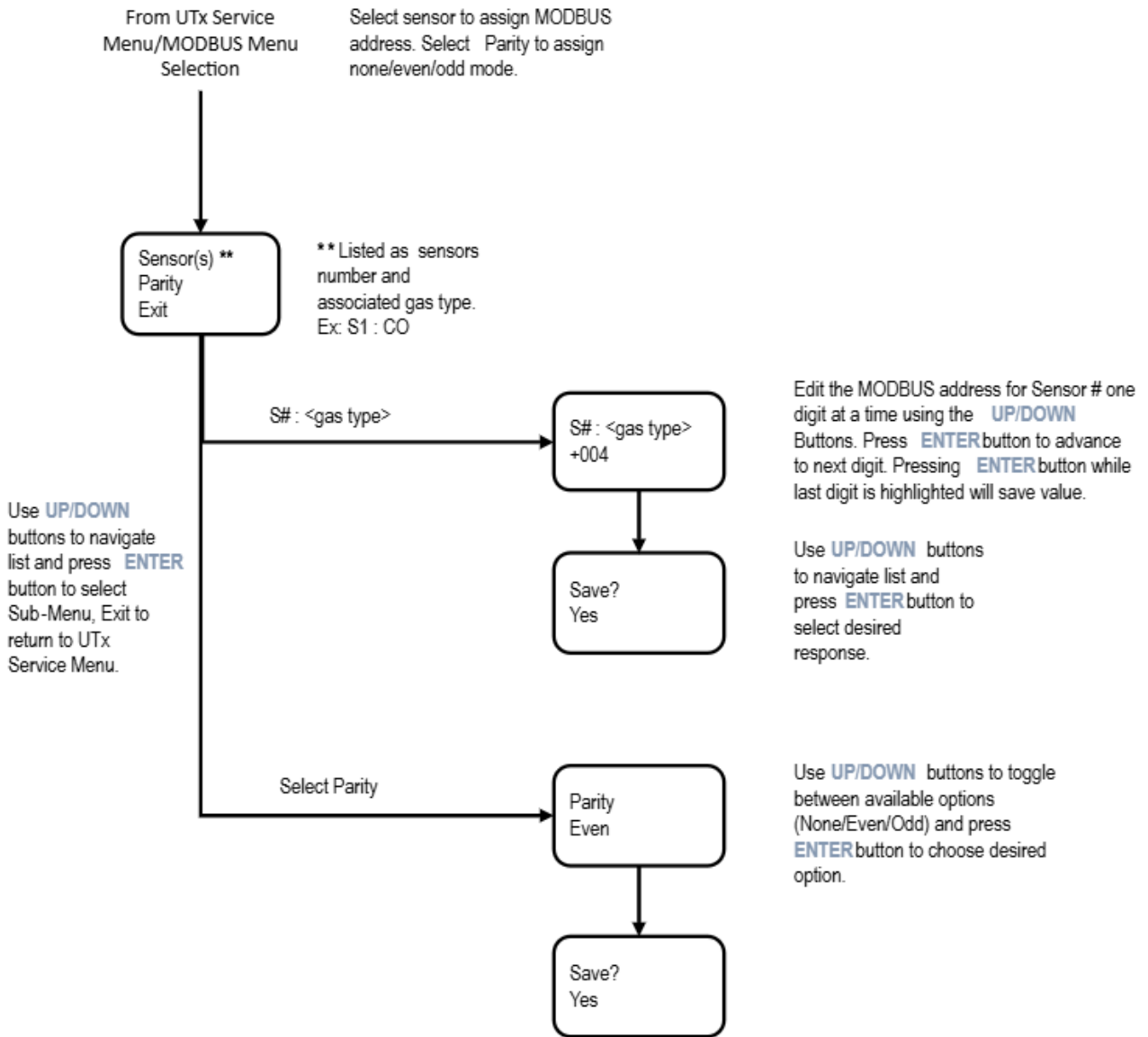
Figure 9-4: Modbus Menu Flow Diagram
