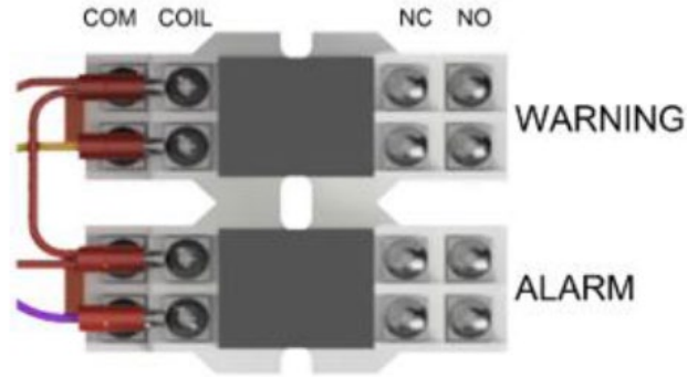
Figure 3-4: Relay Connections
