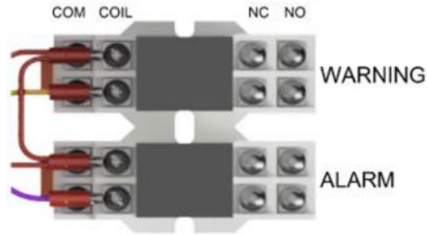
Figure 3-4: Relay Connections
