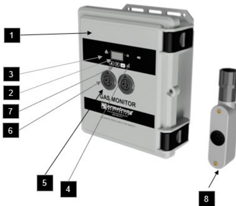
Figure 2-1: External View
