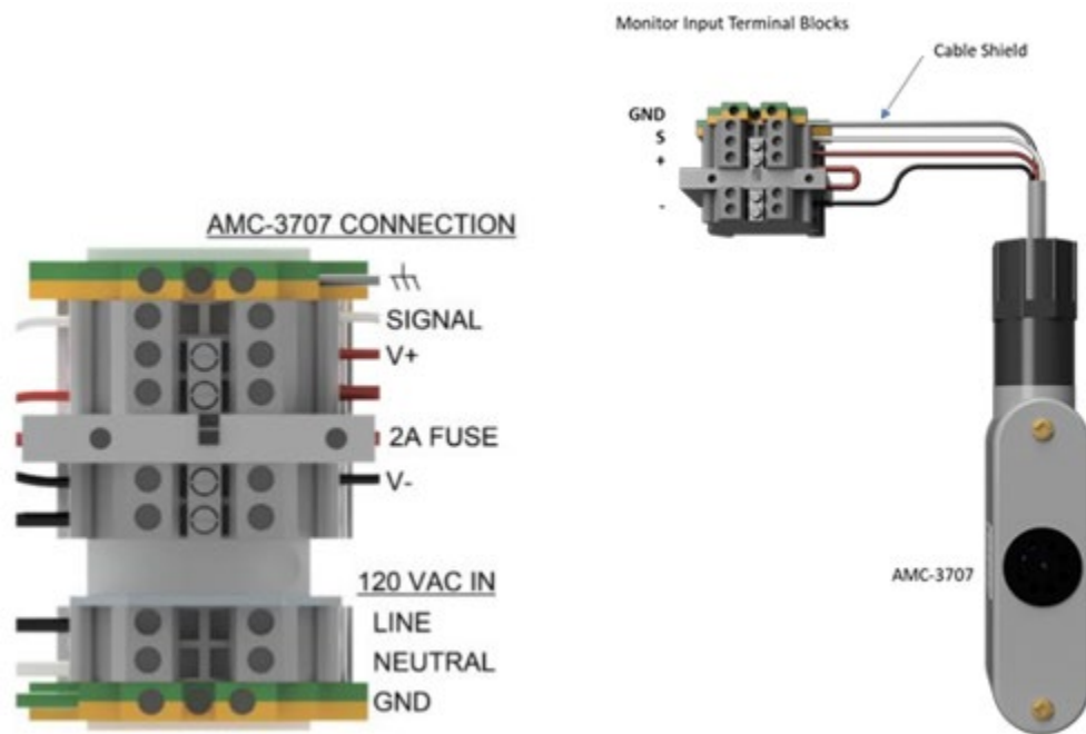
Figure 3-3: Input Terminal Blocks and Wiring to AMC-3707
