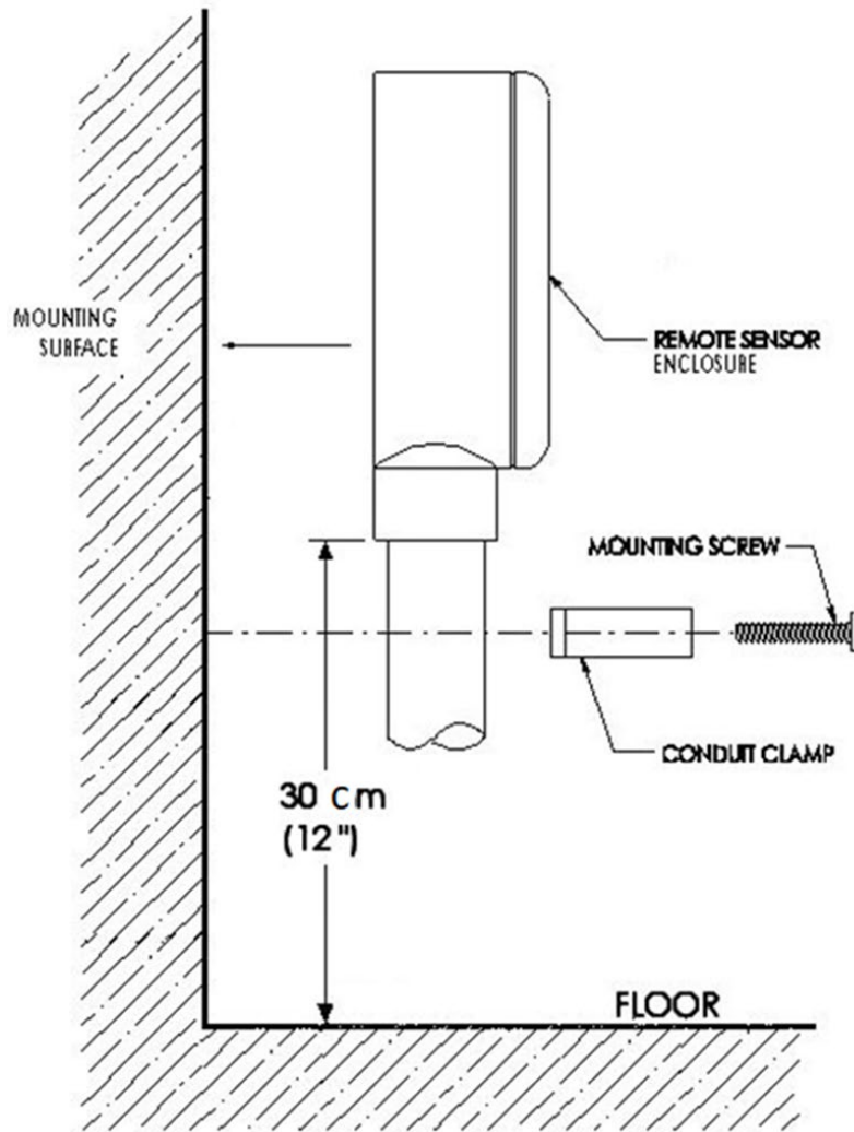
Figure 3-2: AMC-3707 Mounting
