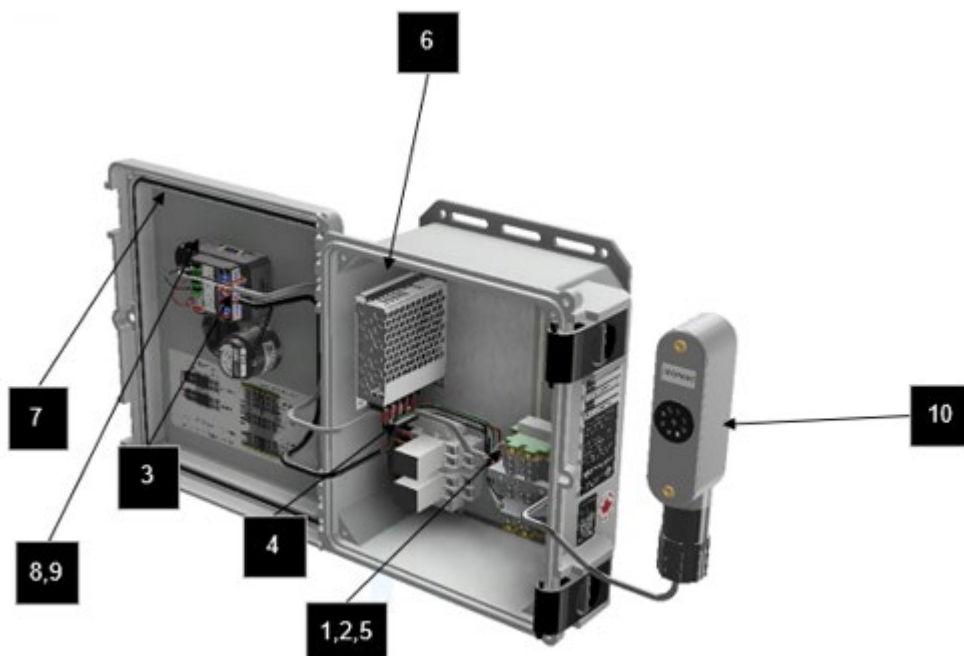
Figure 2-2: Internal View
