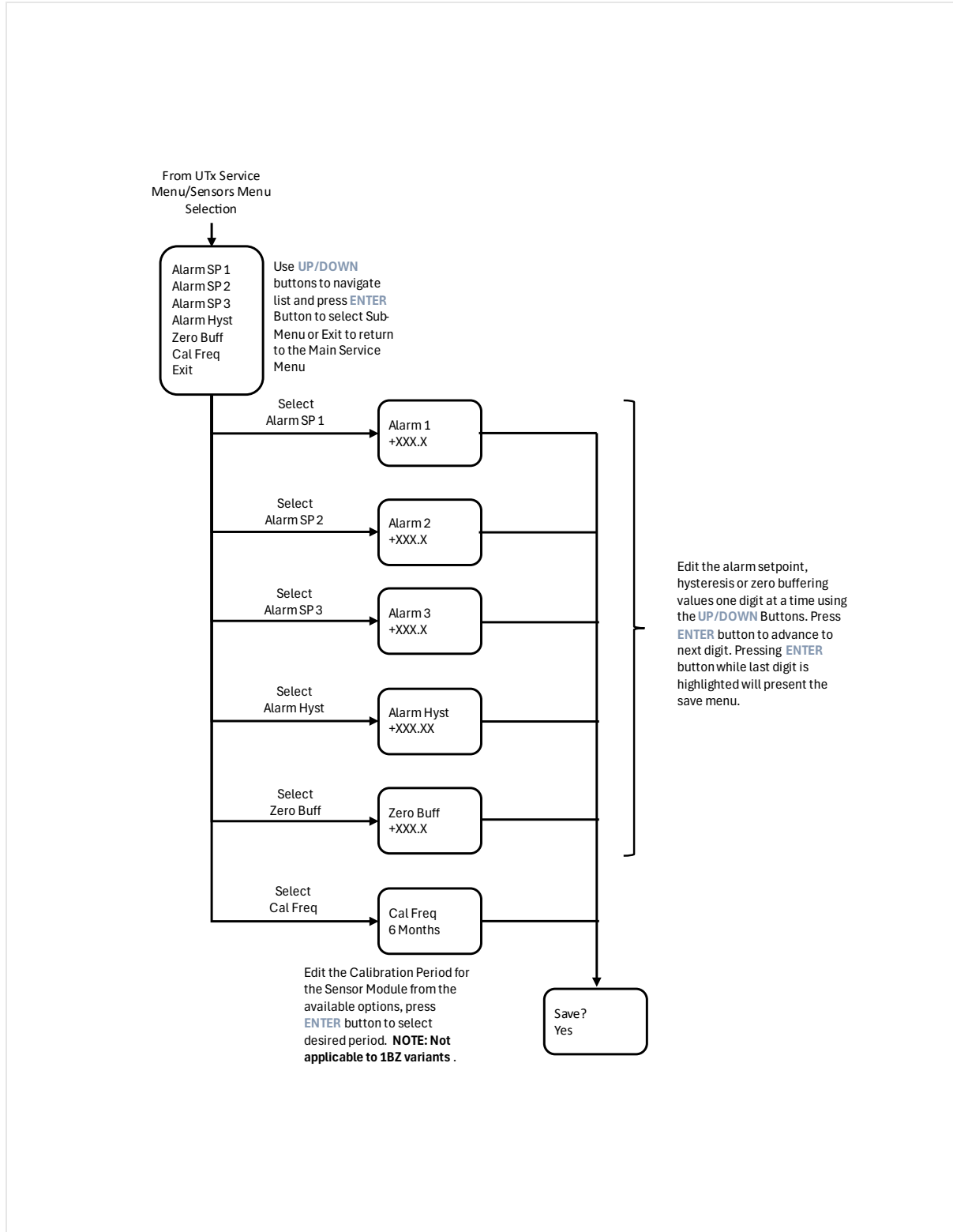
Figure 8-7: Alarm Menu Flow Diagram
