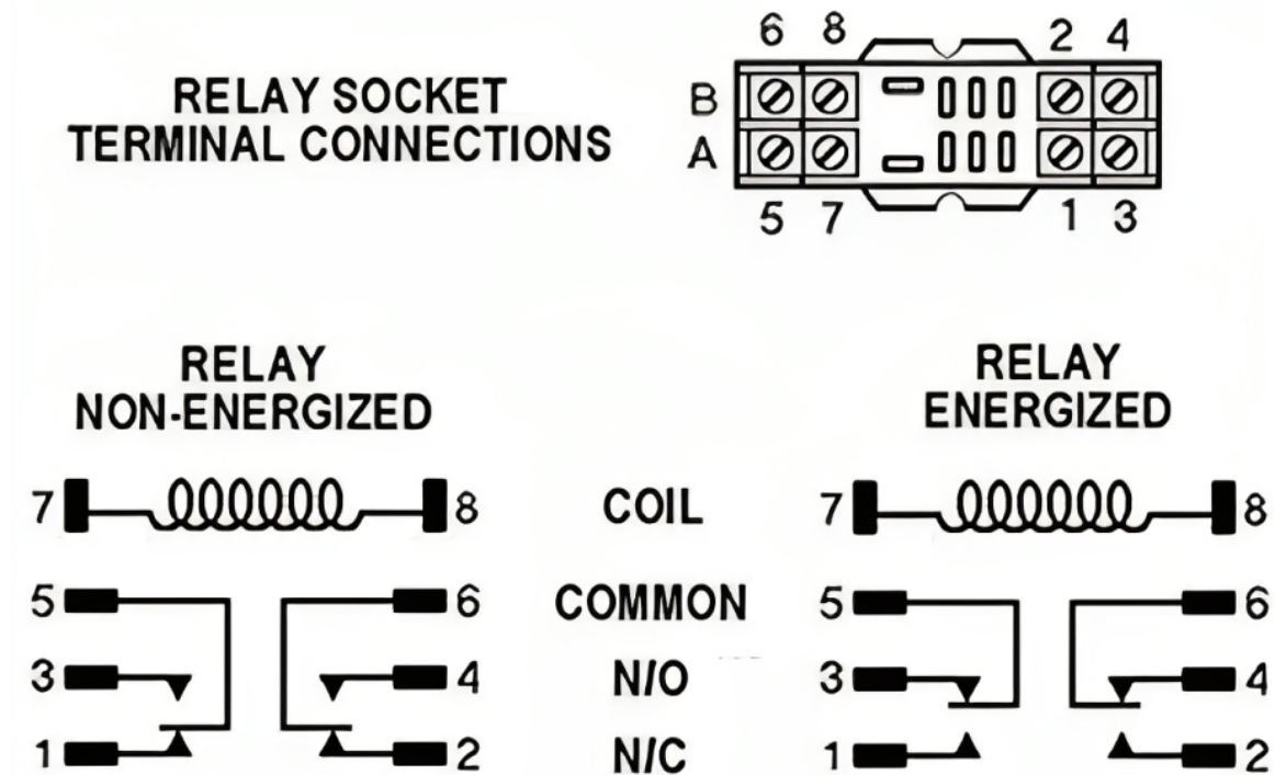
Figure 3-2: Relay Connections
