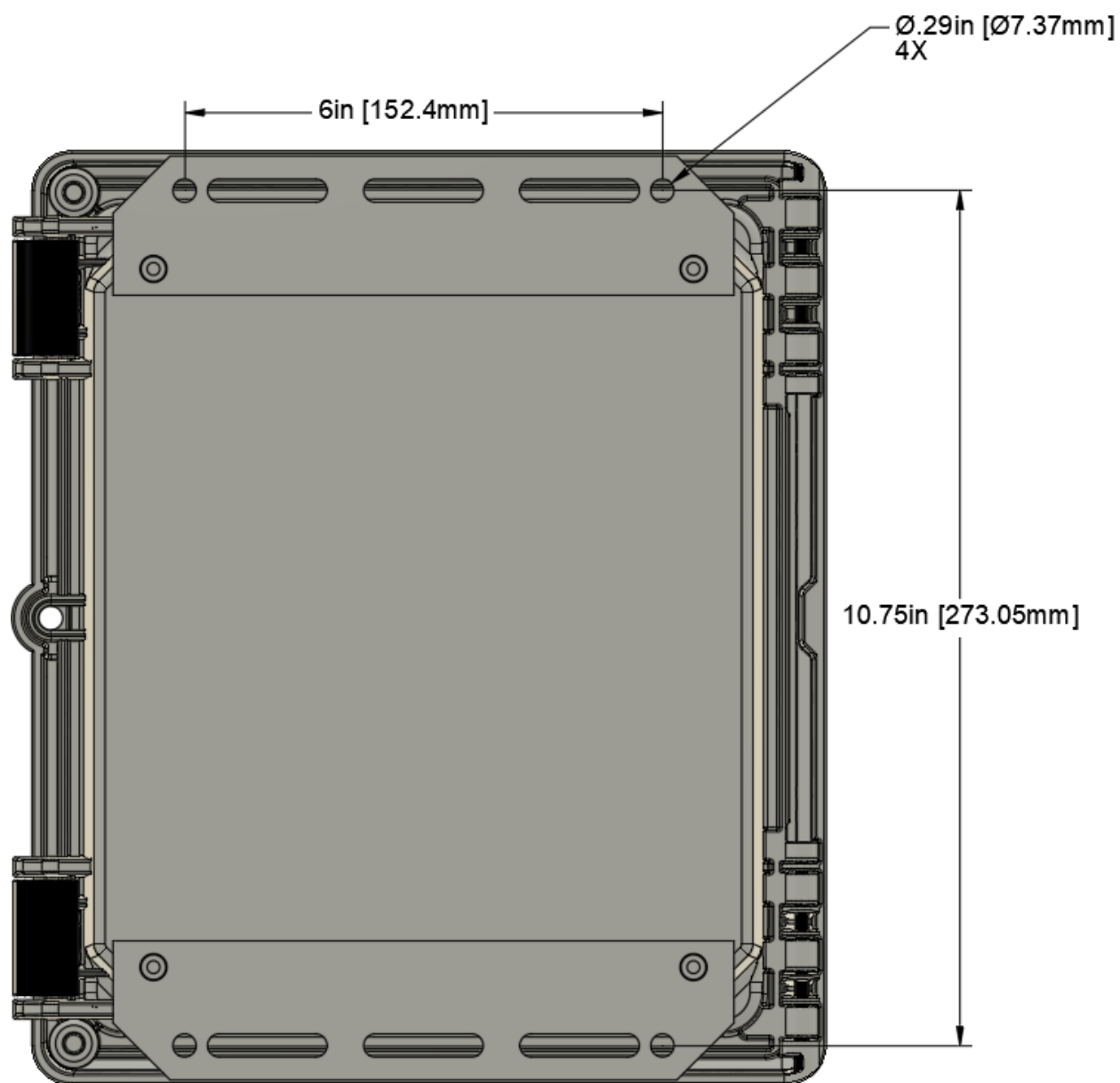
Figure 3-1: Enclosure Mounting
