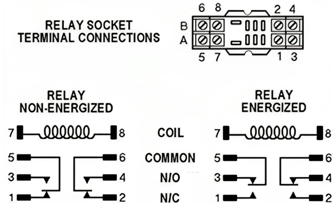
Figure 3-2: Relay Connections
