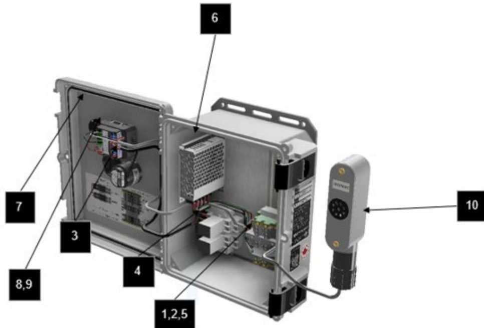
Figure 2-2: Internal View
