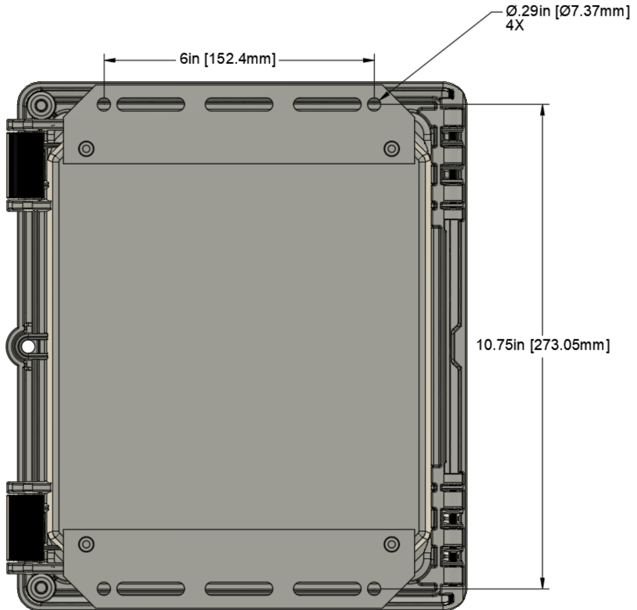
Figure 3-1: Enclosure Mounting
