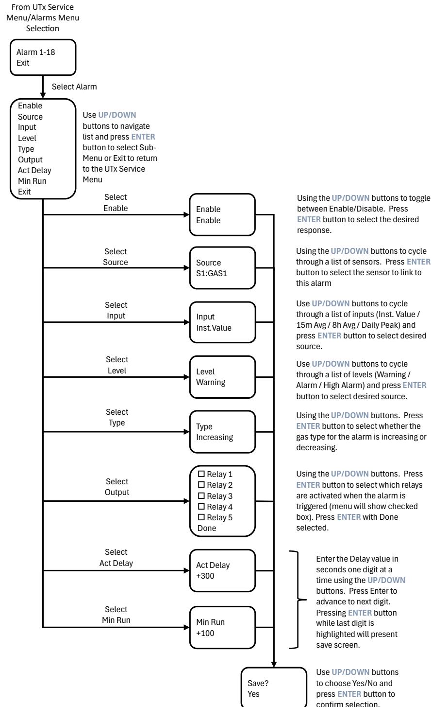
Figure 8-7: Alarm Menu Flow Diagram
