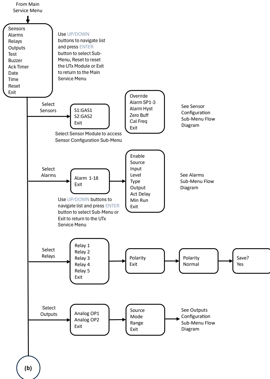
Figure 8-2: UTx Service Menu (a)
