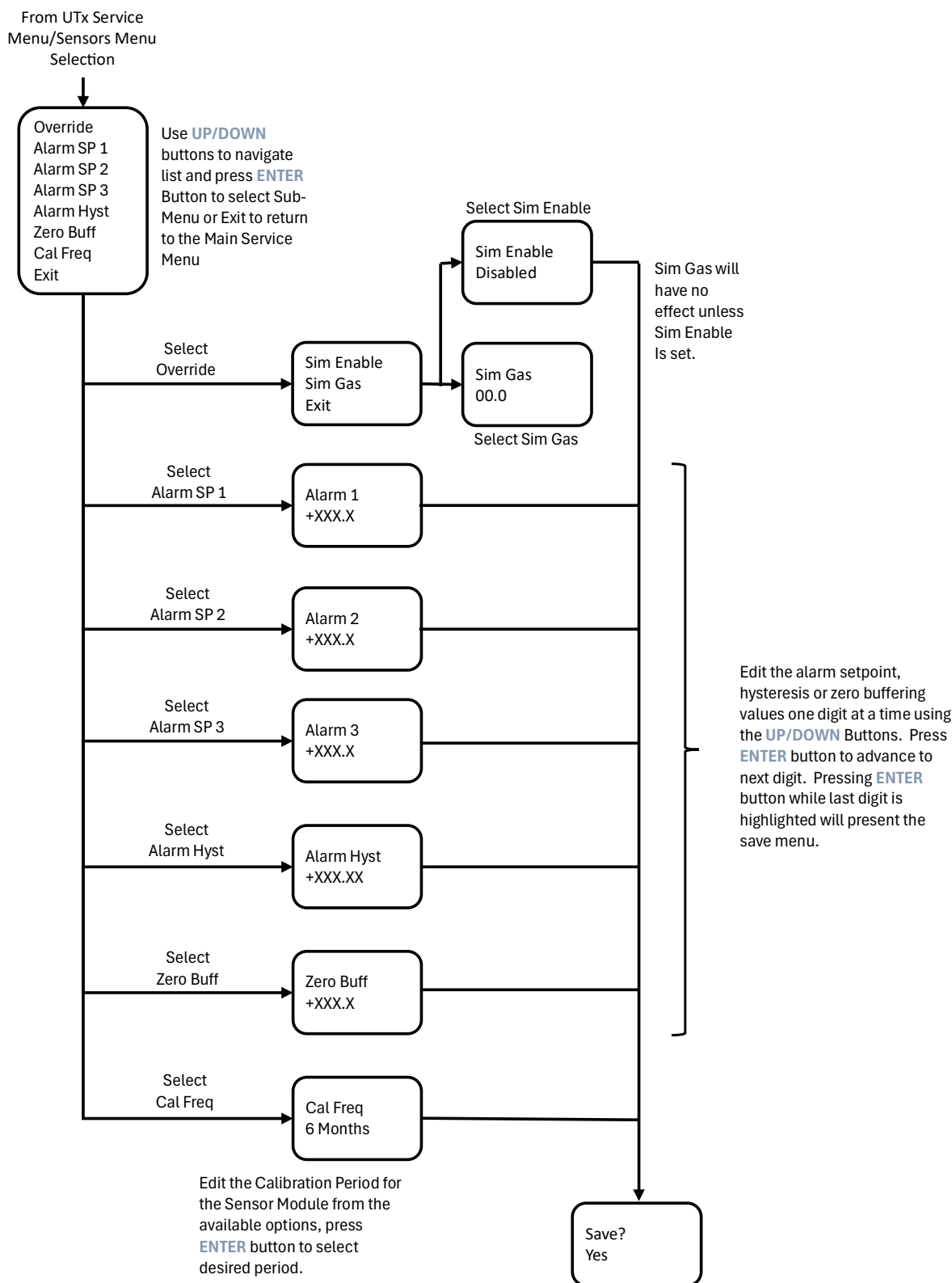
Figure 8-6: Sensor Configuration Menu Flow Diagram
