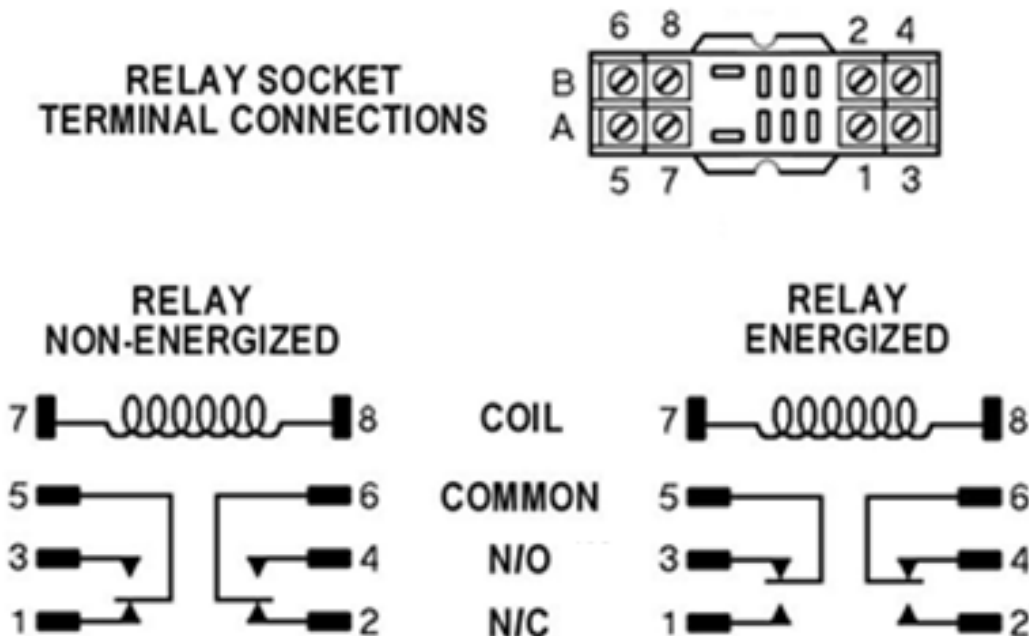
Figure 3-2: Relay Connections
