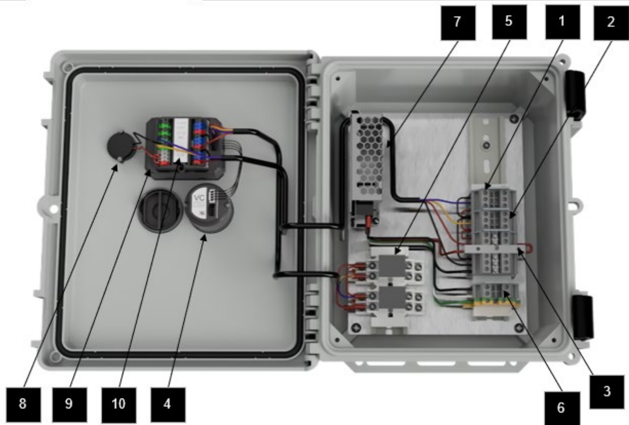
Figure 2-2: Internal View
