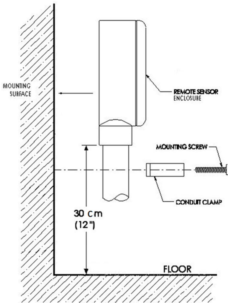
Figure 3-2: AMC-3707 Mounting
