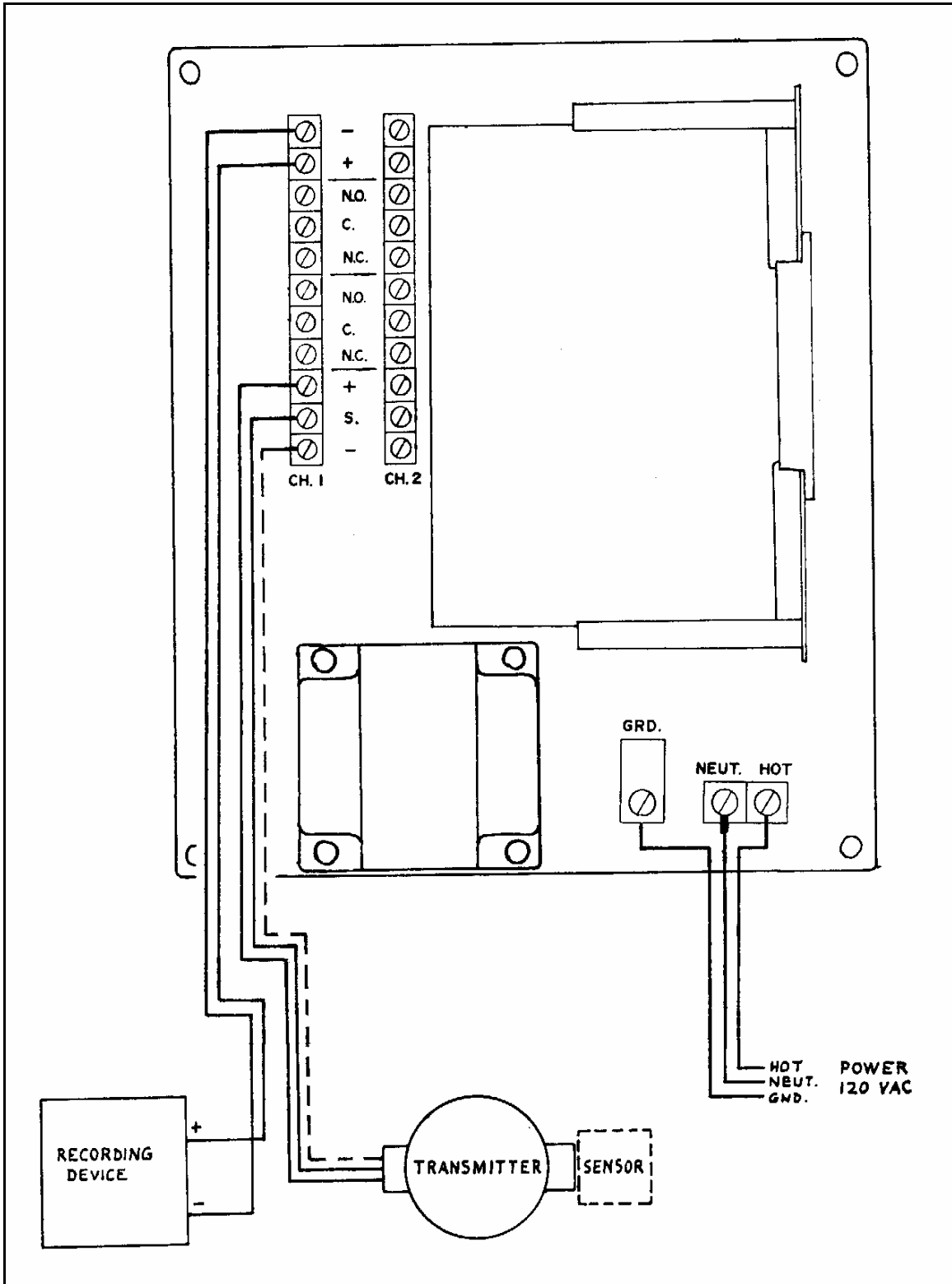
FIGURE 2.2 POWER SUPPLY, TRANSMITTER AND RECORDER CONNECTIONS
