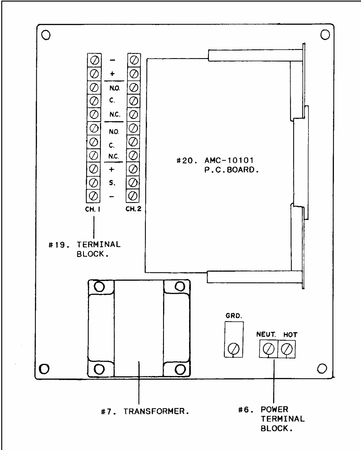
FIGURE 1.3 AMC-1011/1012 MONITOR, INSIDE PANEL
