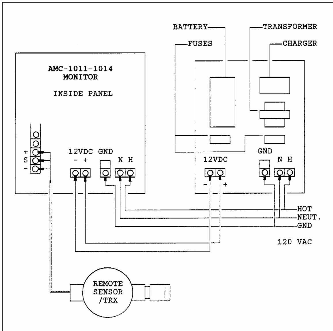
FIELD WIRING LAYOUT FOR AMC-1011/1014 MONITOR WITH BATTERY BACKUP FUNCTION
