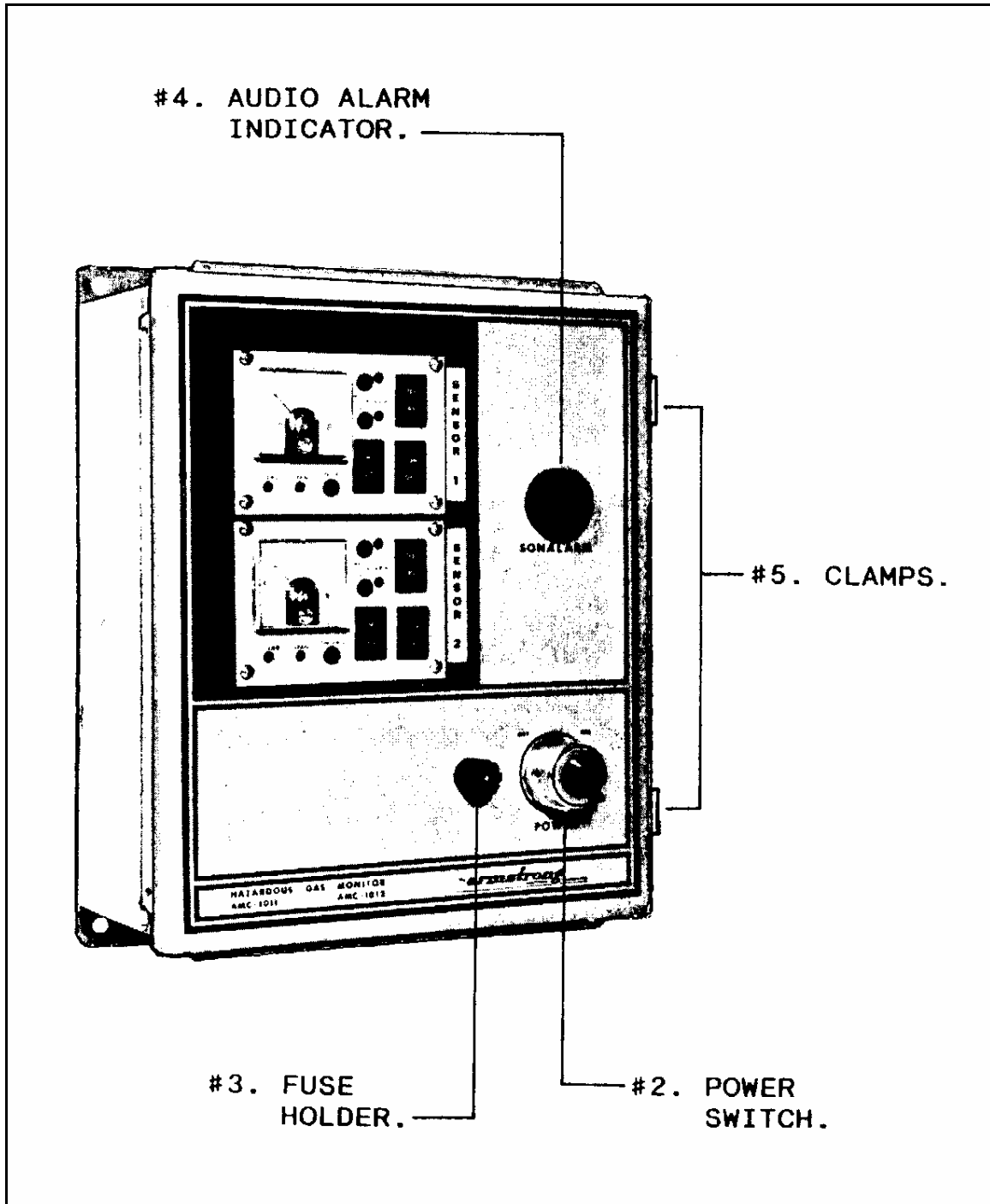
FIGURE 1.1 AMC-1011/1012 MONITOR, FRONT PANEL
