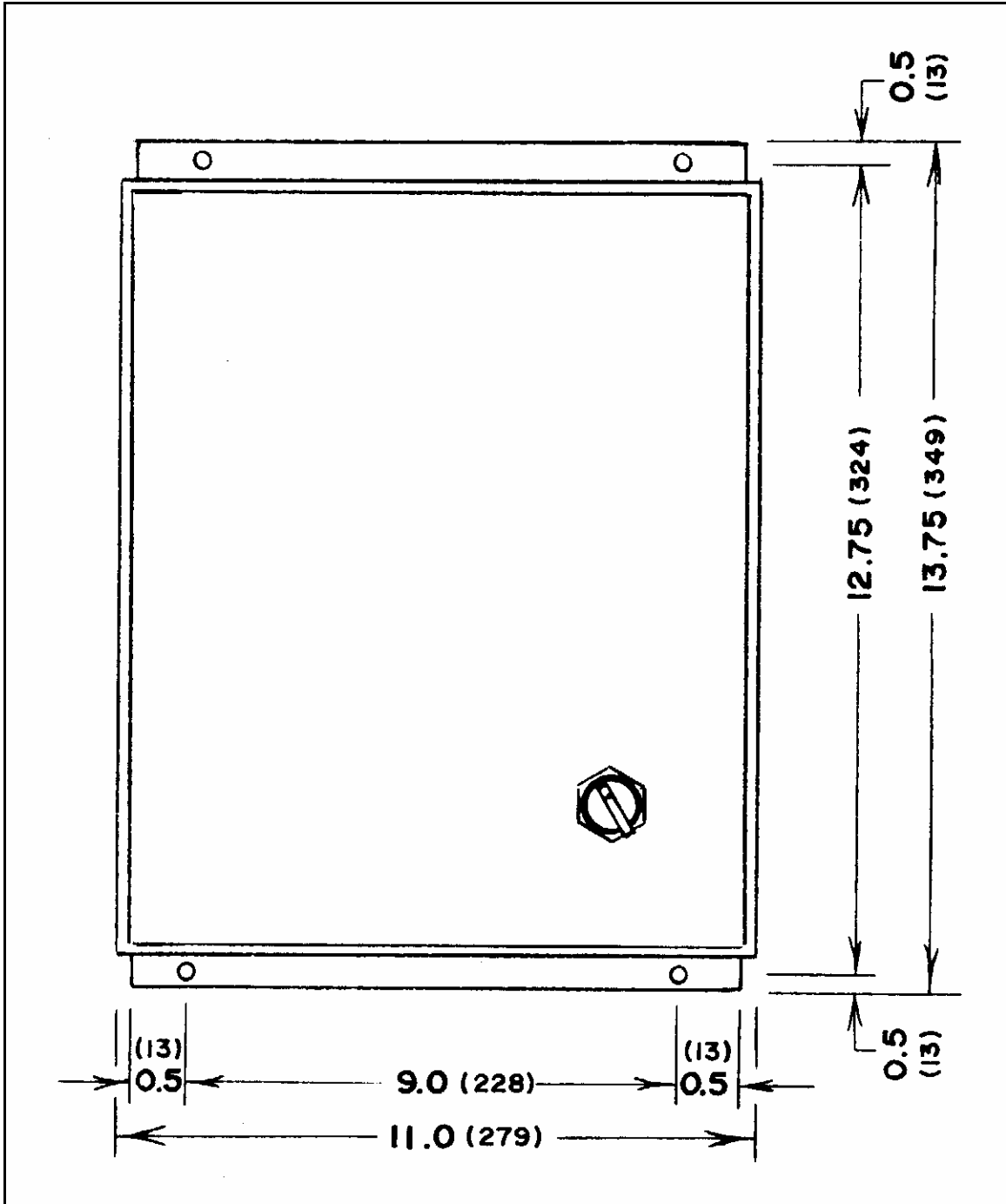
FIGURE 2.1 AMC-1011/1012 MONITOR MOUNTING DIMENSIONS
