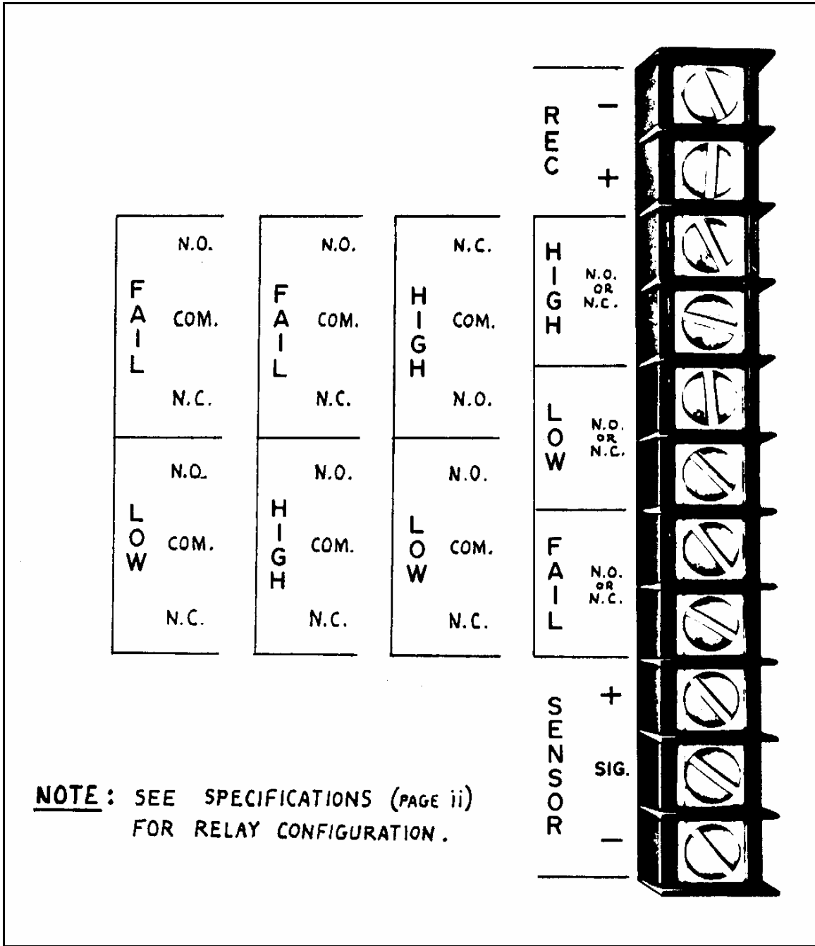
FIGURE 2.3 RELAY WIRING DIAGRAM, SHOWING THE CONTACT ARRANGEMENT FOR THE NON-ALARM CONDITION
