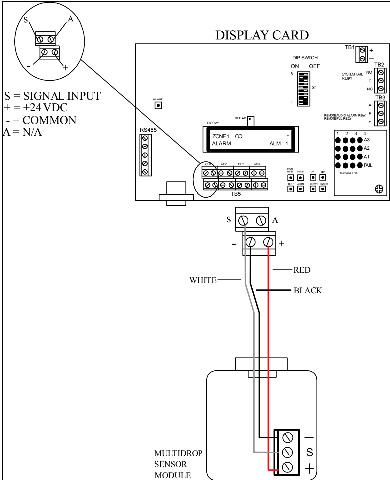
FIGURE 5: Multidrop Sensor Module Terminal Block Connections
