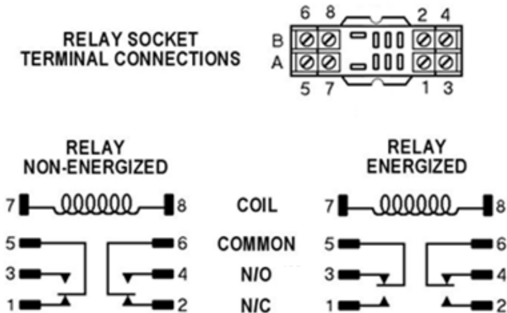
Figure 3-2: Relay Connections
