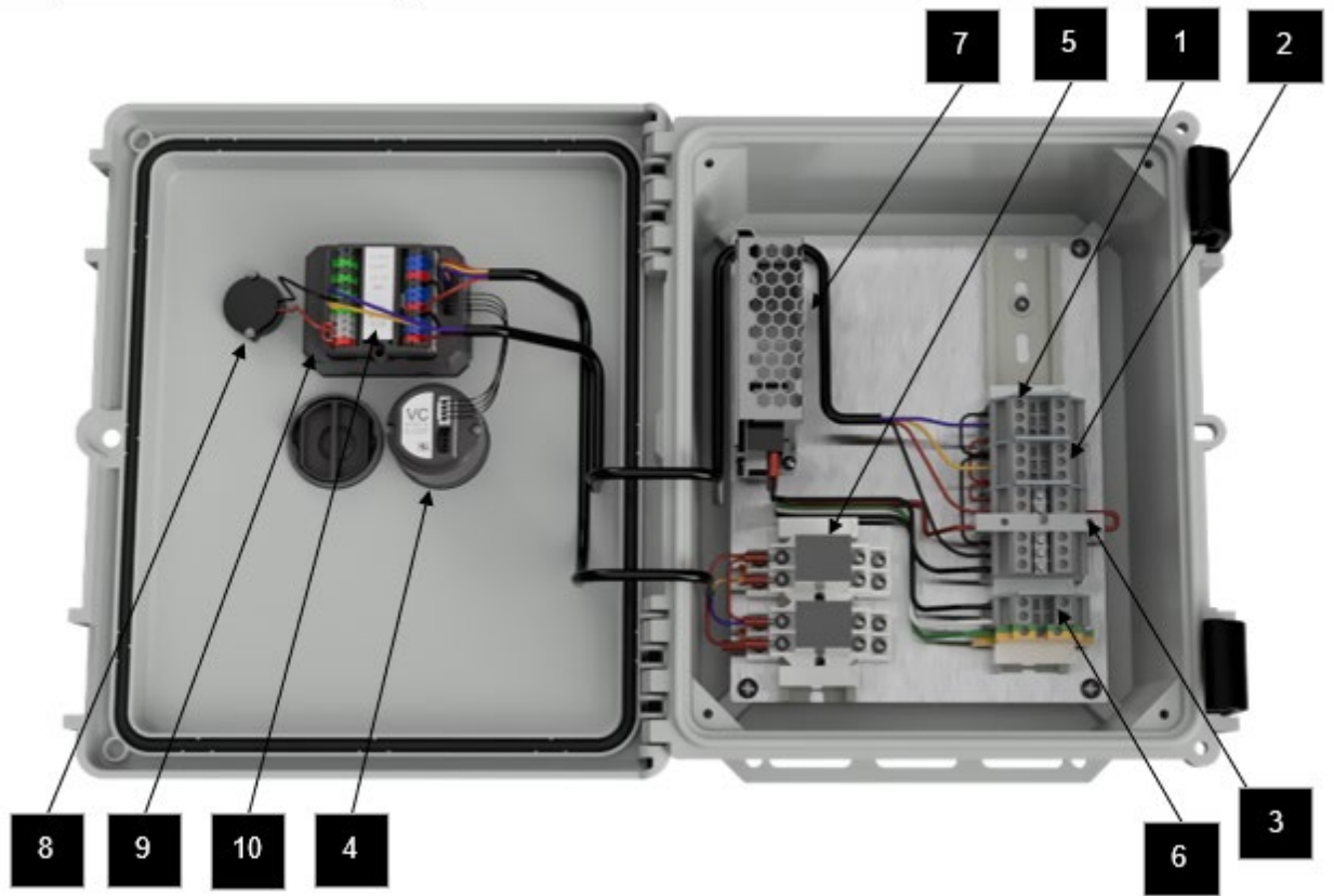
Figure 2-2: Internal View
