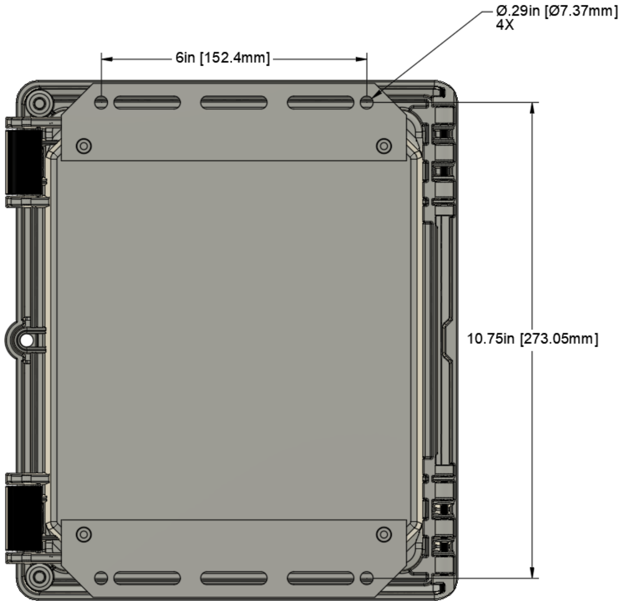
Figure 3-1: Enclosure Mounting
