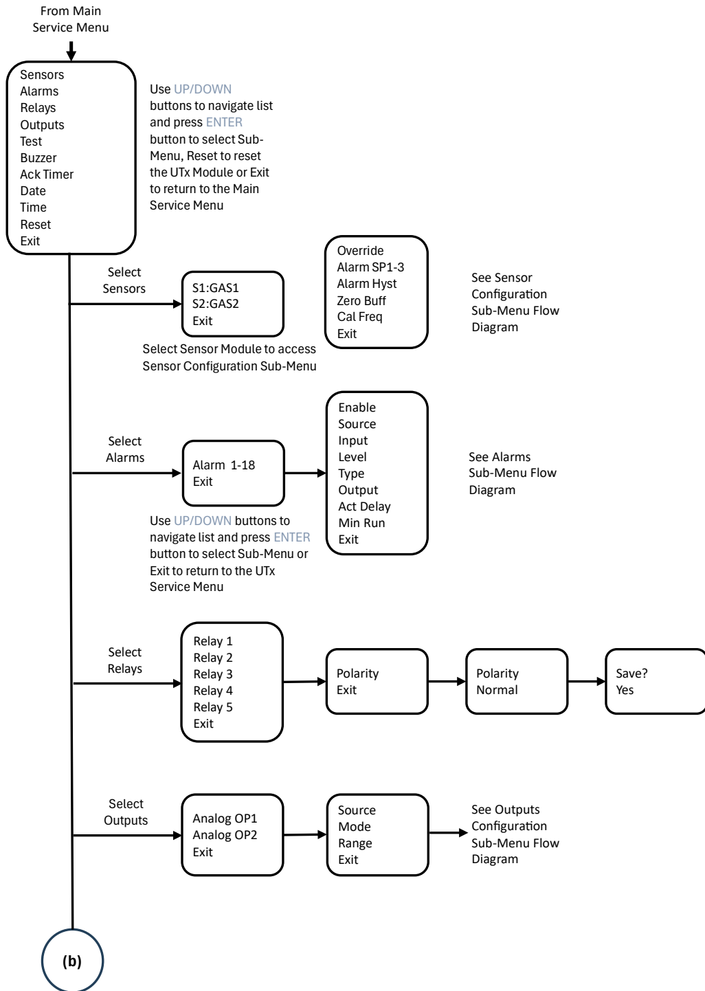
Figure 8-2: UTx Service Menu (a)
